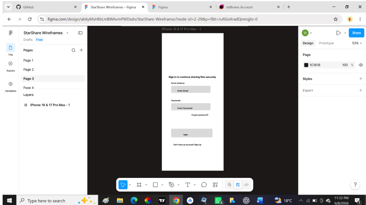
Figure 3: Login screen Wireframe
